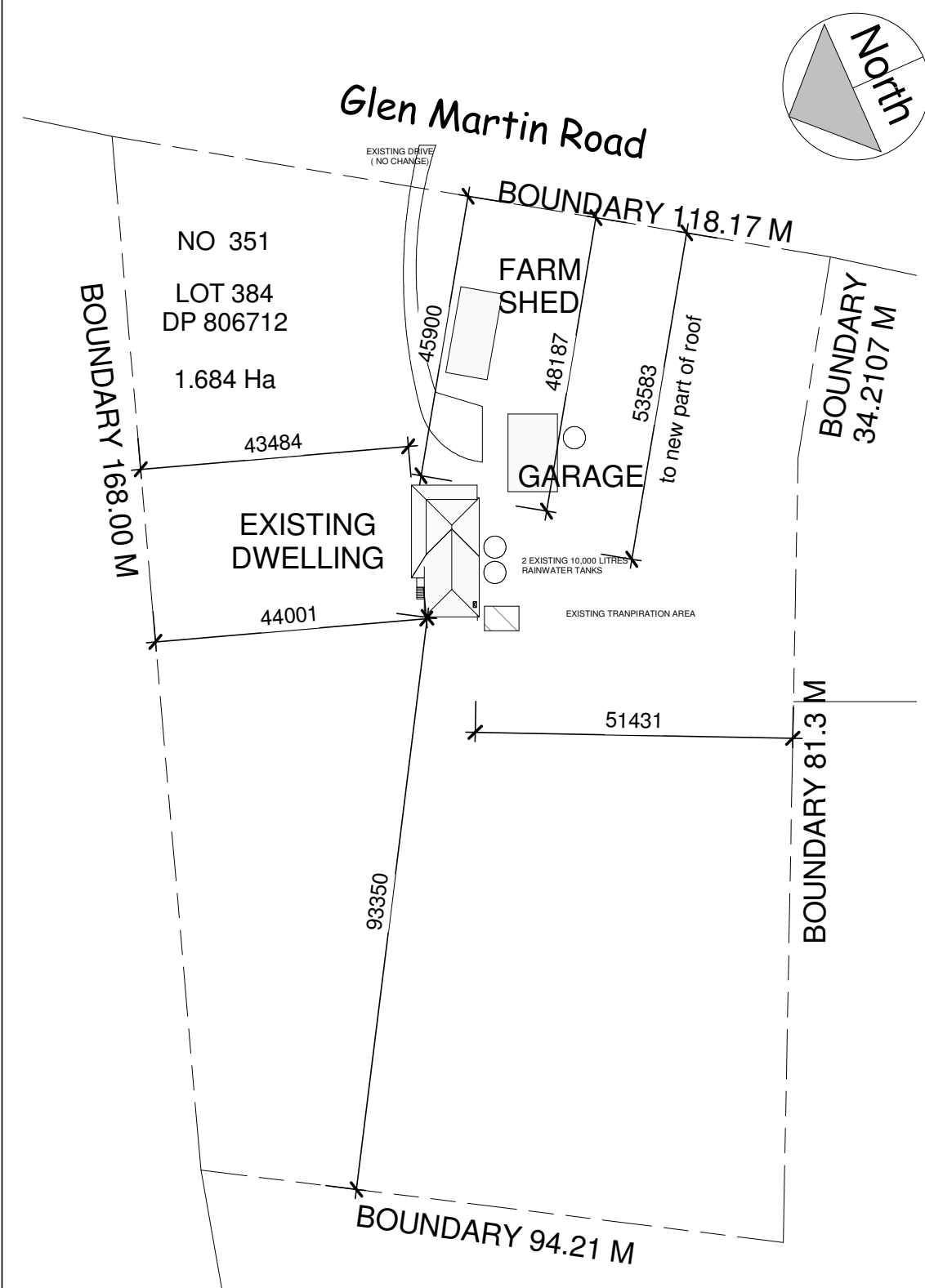
1 Site Plan - Proposed 1 : 1000
