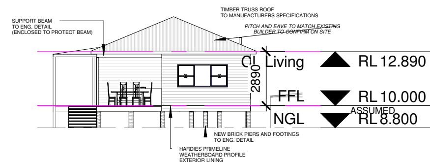
3 Rear Elevation 1 : 200
